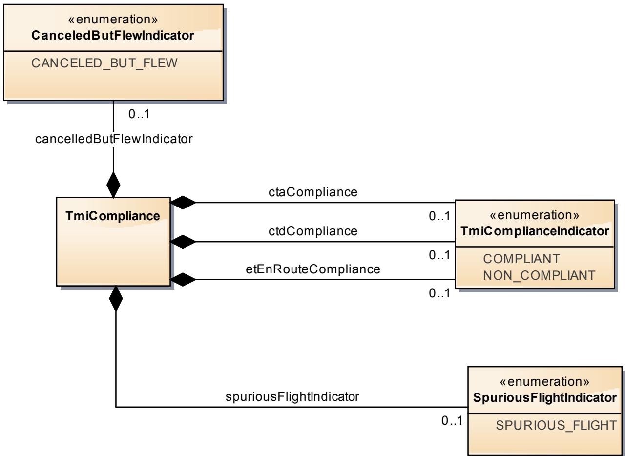
Figure 18: NasTmiCompliance
