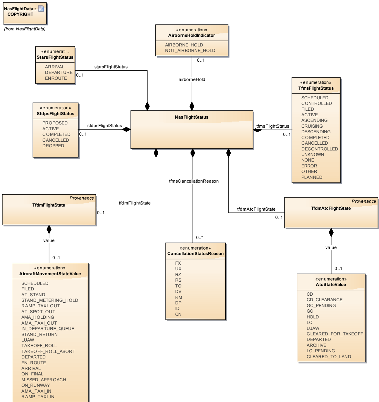
Figure 16: NasStatus
