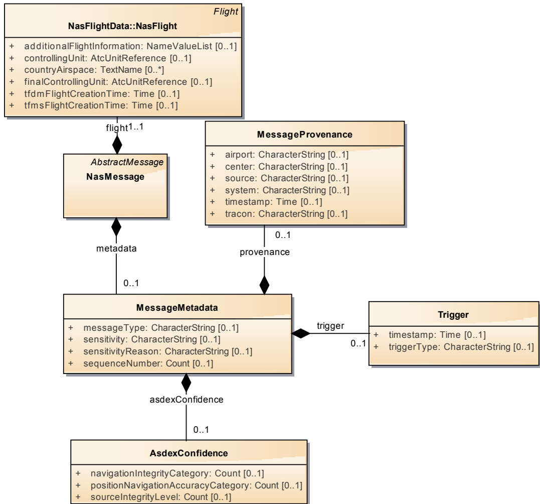
Figure 13: NasMessage
