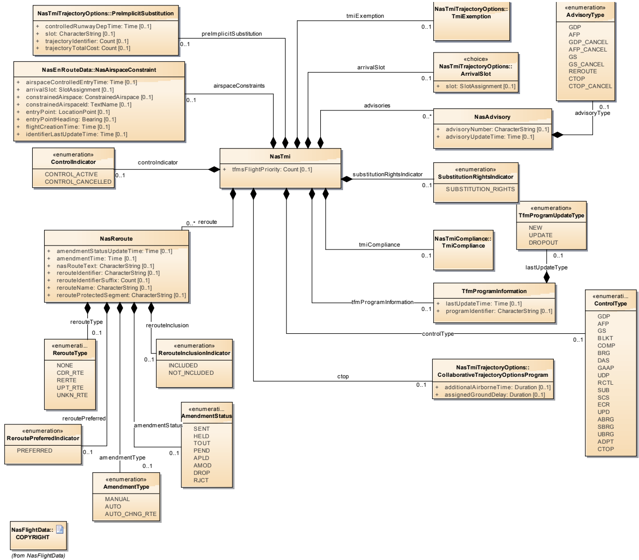
Figure 19: NasTmiData
