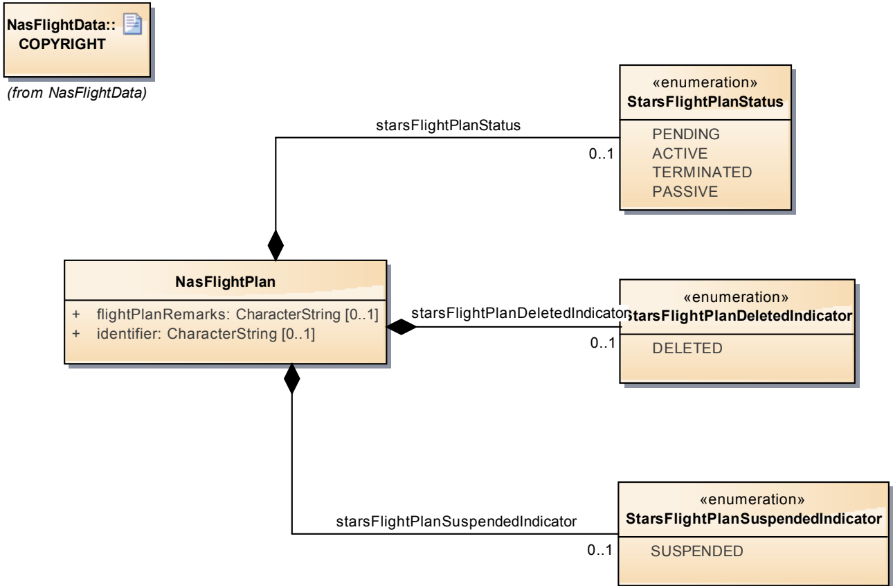
Figure 11: NasFlightPlan
