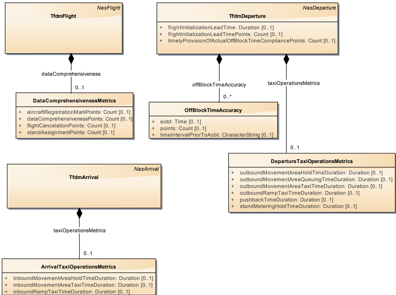
Figure 17: NasTfdm
