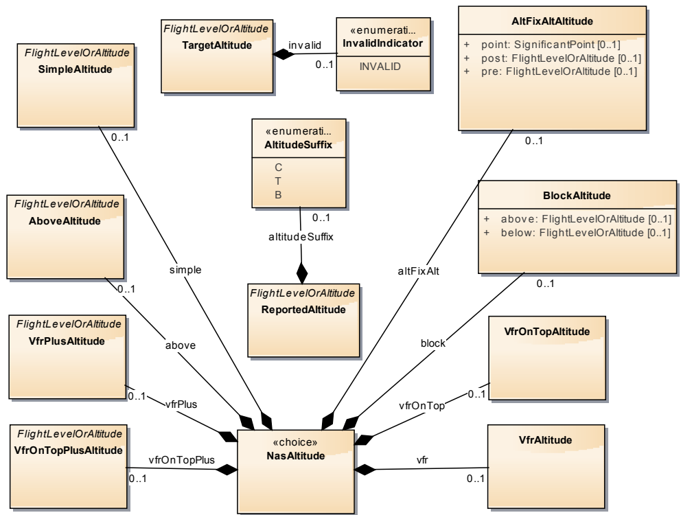
Figure 3: NasAltitude
