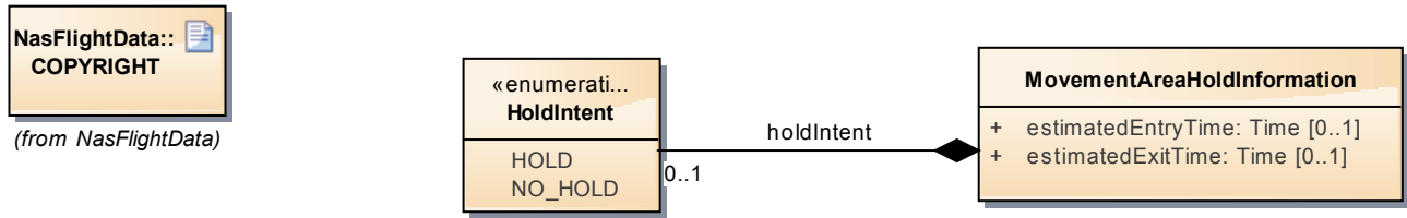
Figure 10: NasFlightIntent
