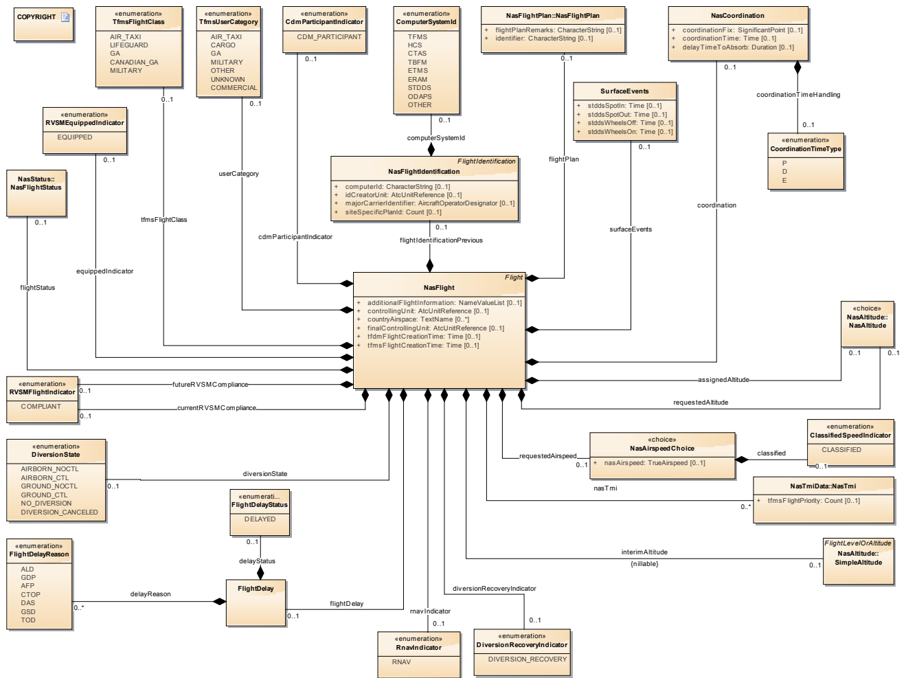
Figure 9: NasFlightData
