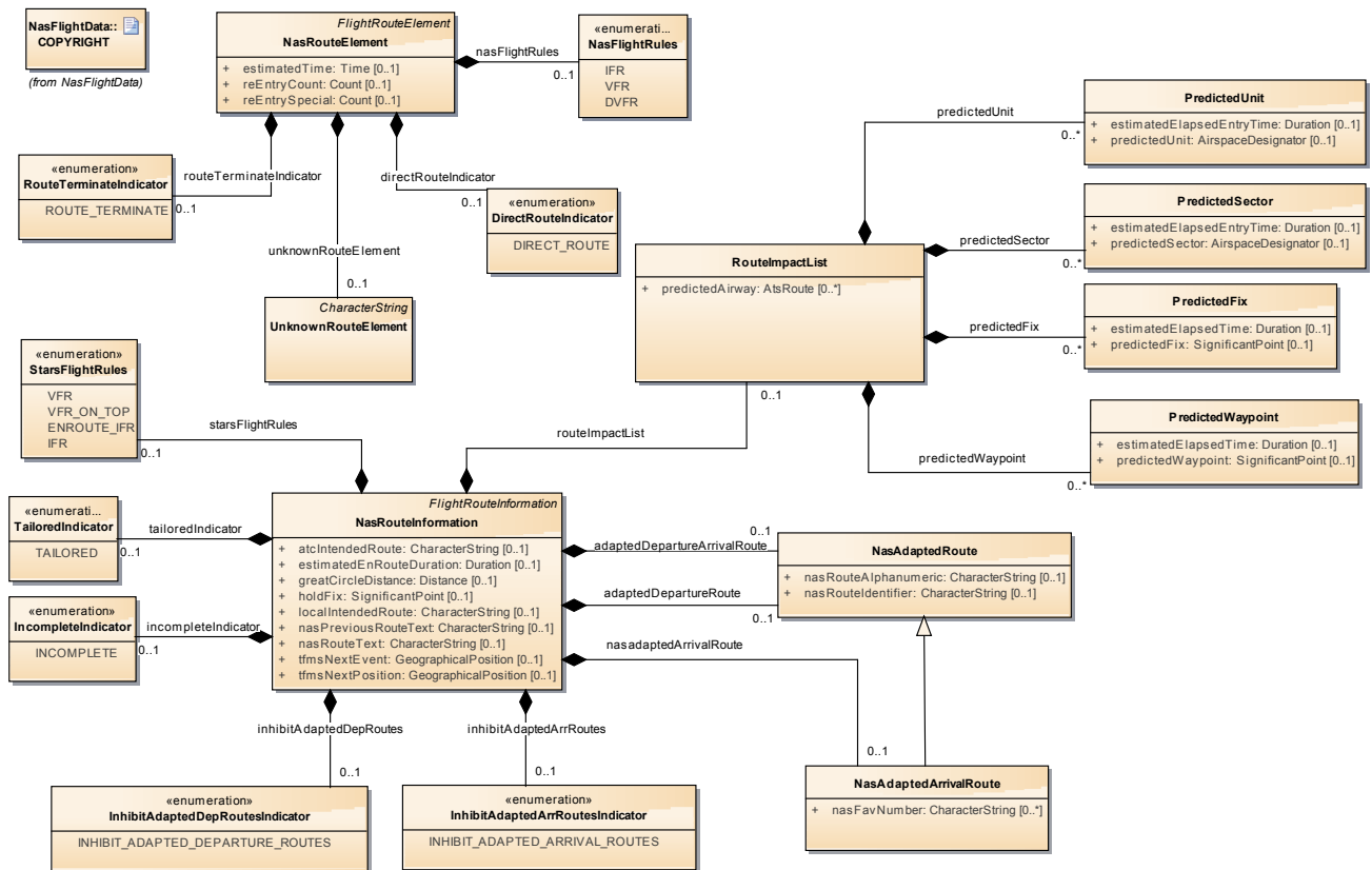
Figure 15: NasRoute
