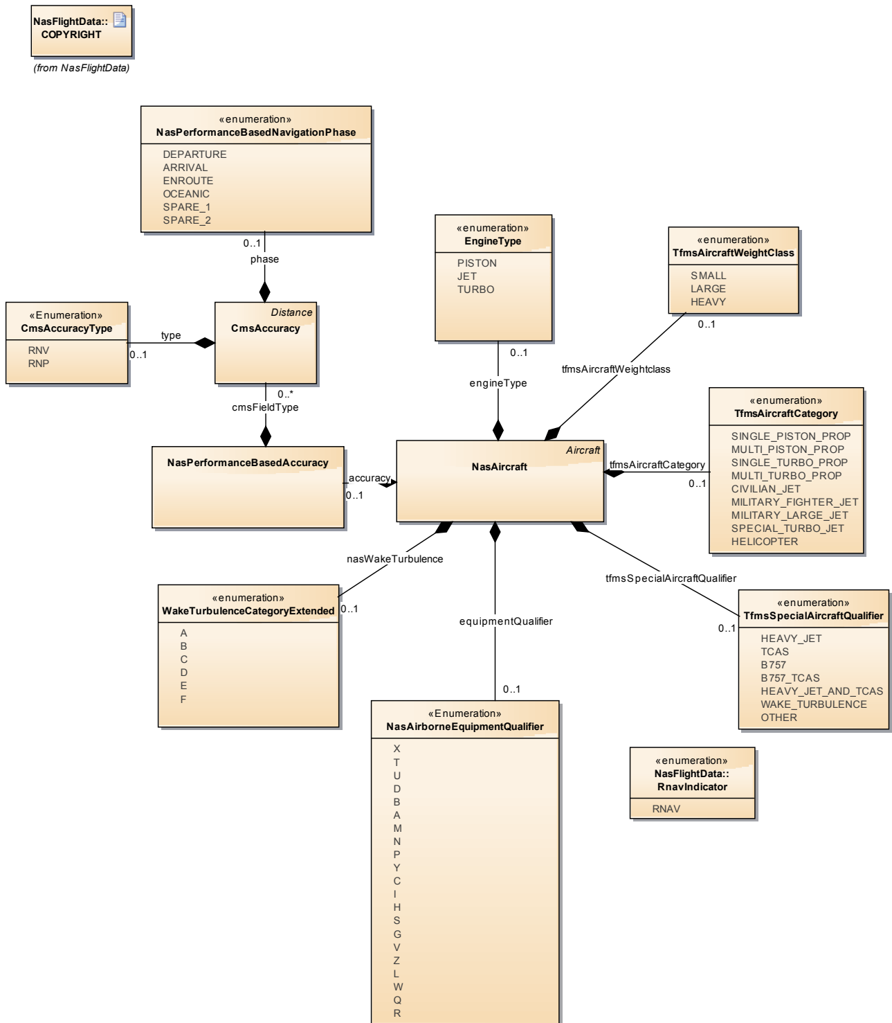
Figure 1: NasAircraft
