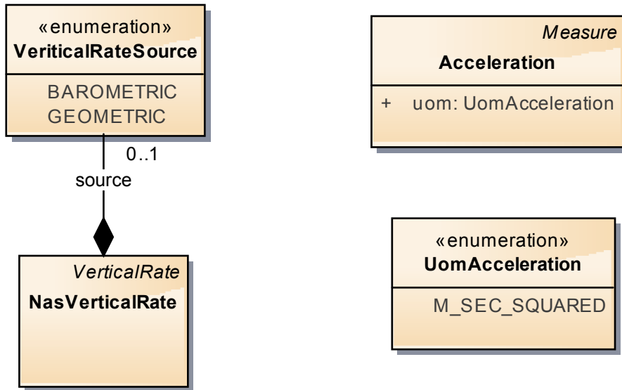
Figure 12: NasMeasures
