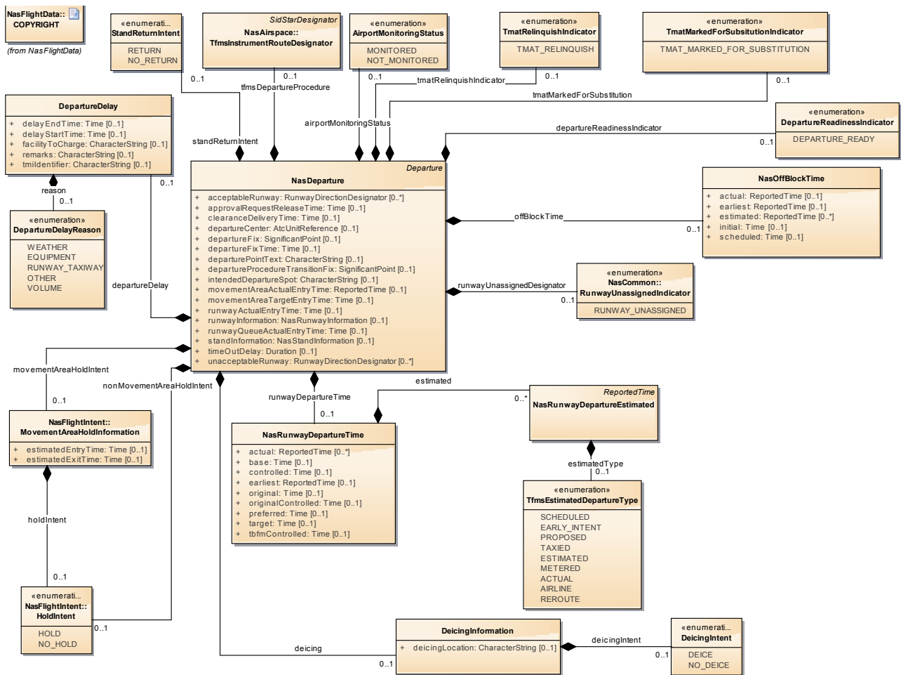
Figure 7: NasDeparture
