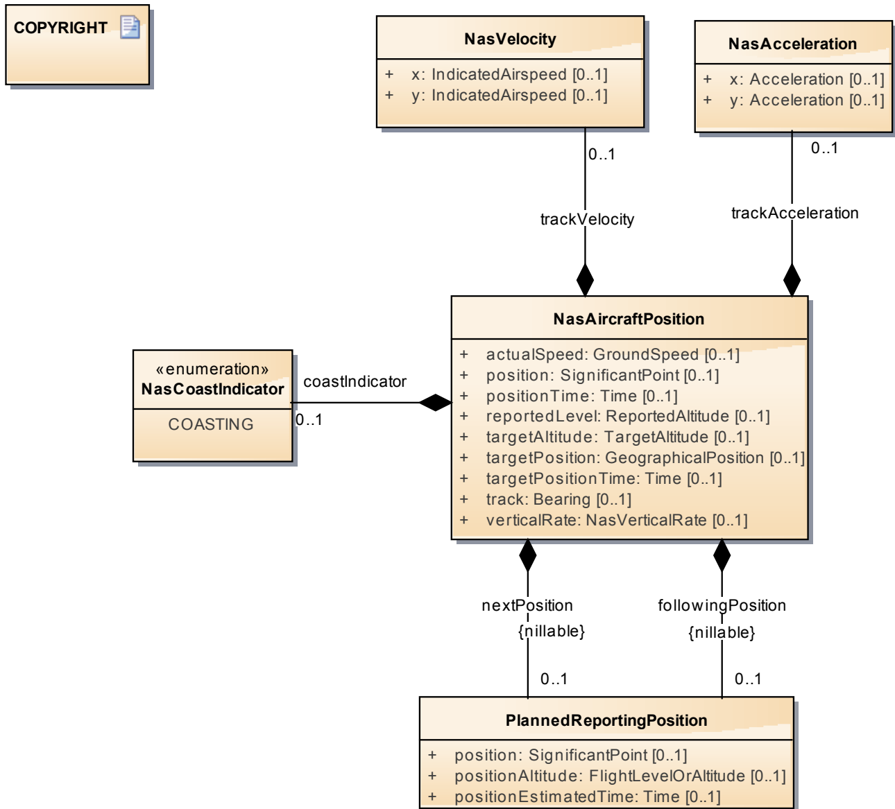
Figure 14: NasPosition
