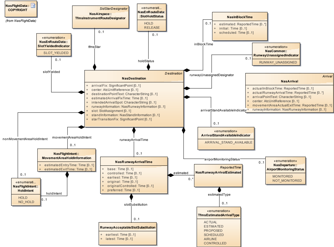
Figure 4: NasArrival
