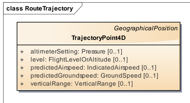
Figure 4 - Inheritance Notations
